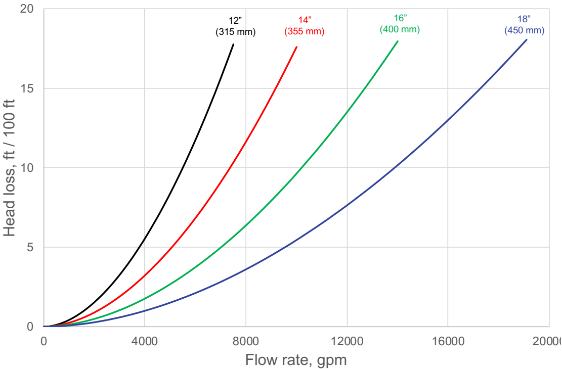
Pressure Loss vs. Flow Rate 12" thru 18", SDR 11
