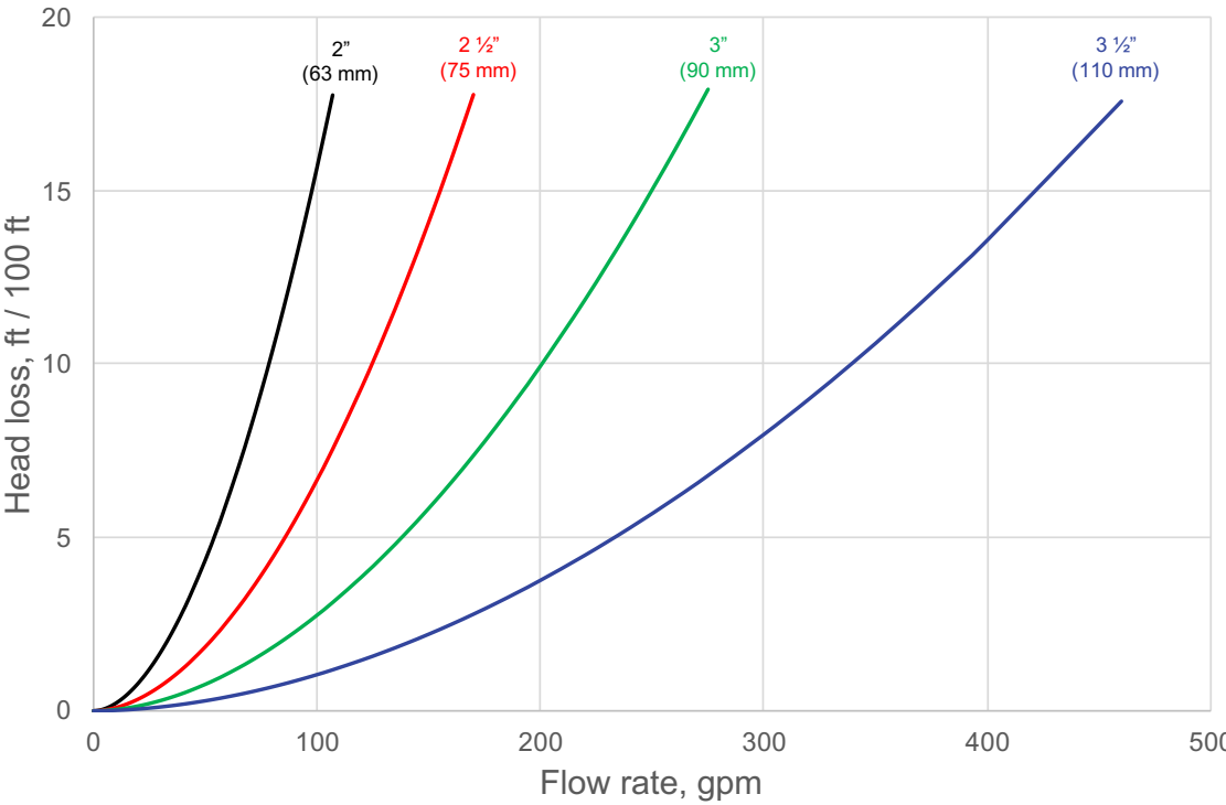
Pressure Loss vs. Flow Rate 2" thru 3-1/2", SDR 11
